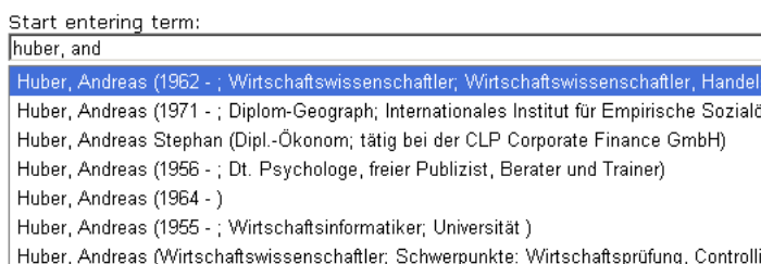
FIG. 2. Extended preferred labels for personal name authority
