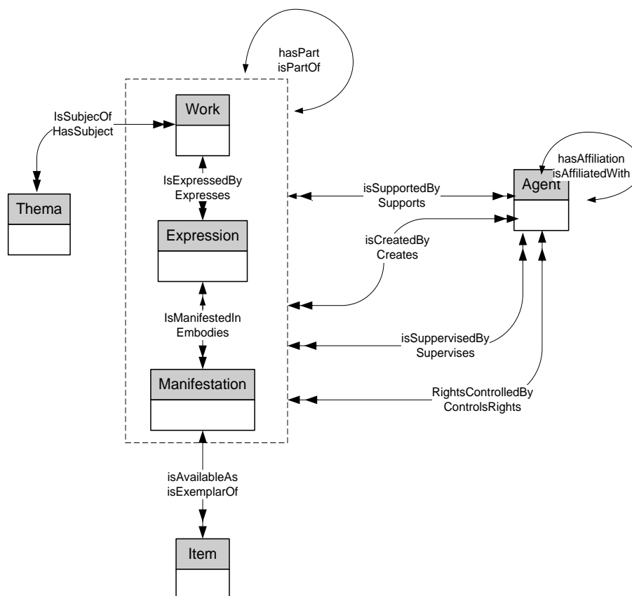
FIG. 6. General DCAP Domain Model
